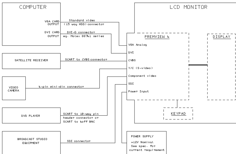
Installation Example
