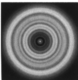
Figure 7-3 A collimated telescope should appear symmetrical with the central obstruction centered in the star's diffraction pattern.
