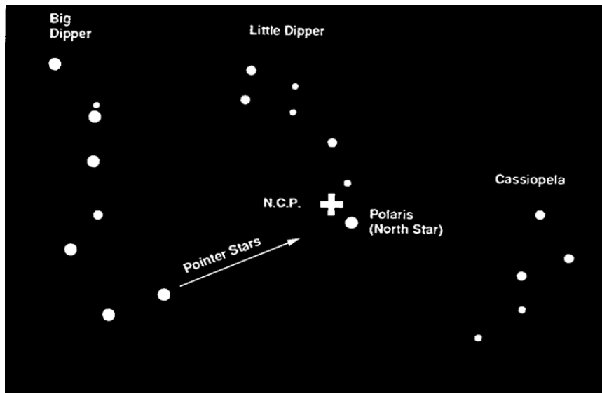
Figure 7-6 The two stars in the front of the bowl of the Big Dipper point to Polaris which is less than one degree from the true (north) celestial pole. Cassiopeia, the "W" shaped constellation, is on the opposite side of the pole from the Big Dipper. The North Celestial Pole (N.C.P.) is marked by the "+" sign.
