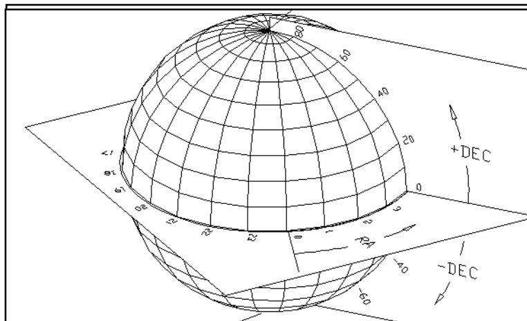
Figure 7-1 The celestial sphere seen from the outside showing R.A. and DEC.
