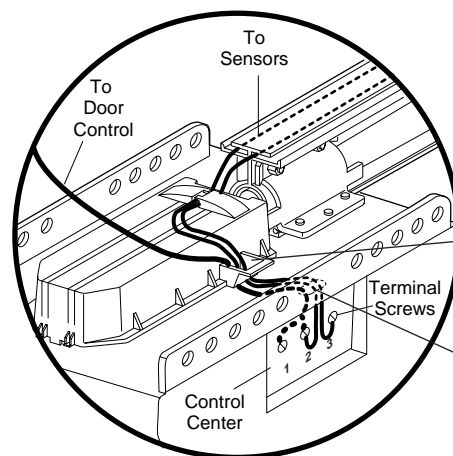
Figure 4 WIRING TO CONTROL CENTER
