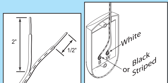
FIG. 3-2 Splitting and stripping.
