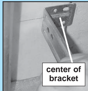
FIG. 4-2 Mounting brackets.
