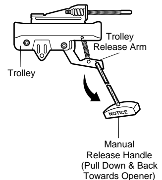
Lockout position
