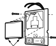
Figure 1 STANDARD INSTALLATION
