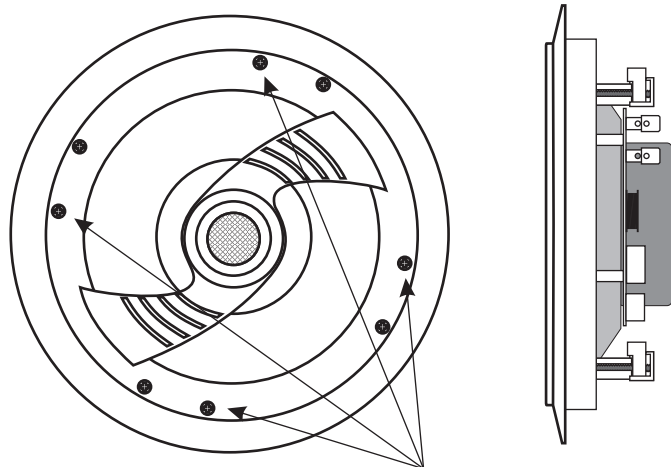
Mounting screws (4)
