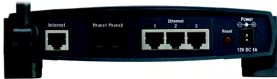
Figure 3-1: Back Panel
