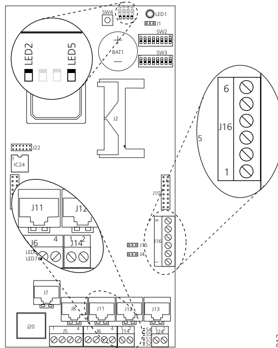
Figure 2. Board description with components described in this chapter.
