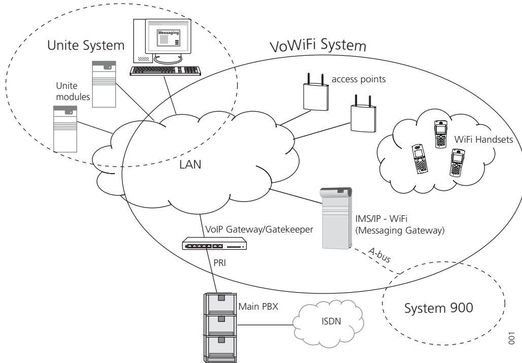
Figure 1. IMS/IP-WiFi connected to the LAN
