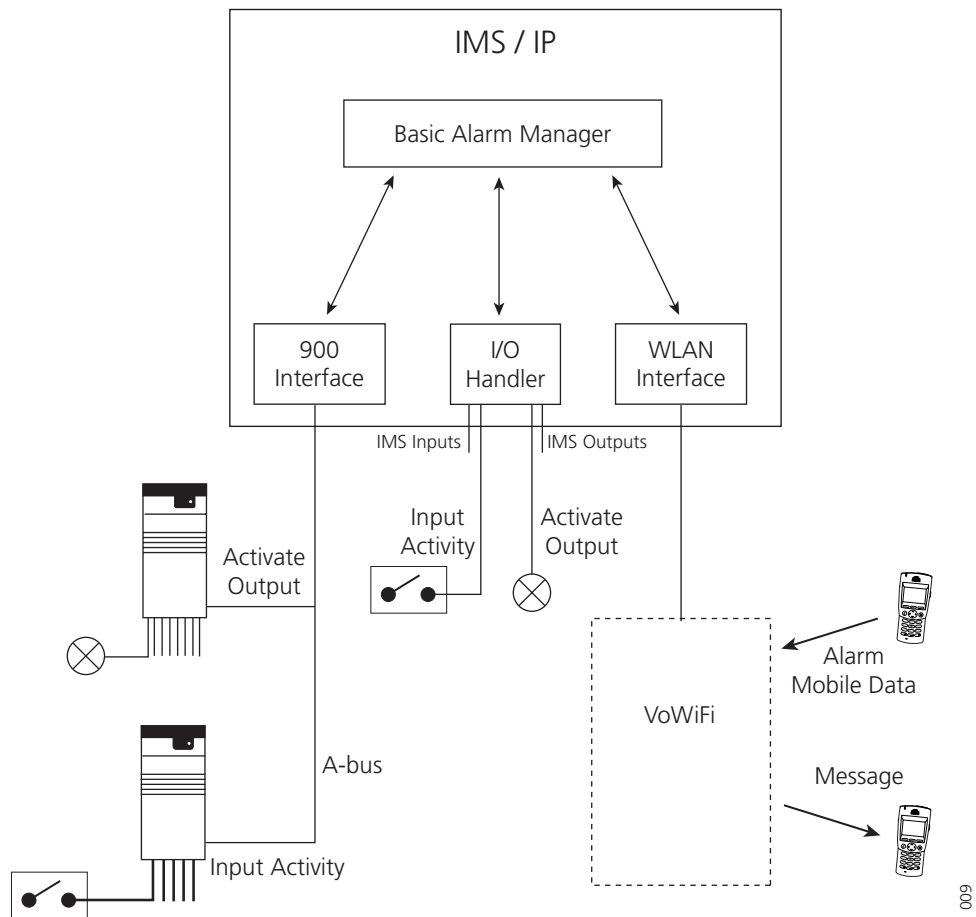
Figure 4. Communication flow for the Basic Alarm Manager and external systems.
