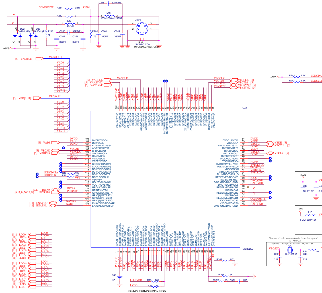
B - 12 LVDS Interface (SiS302LV) (71-D4000-D04)
