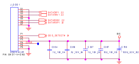
SATA ODD
