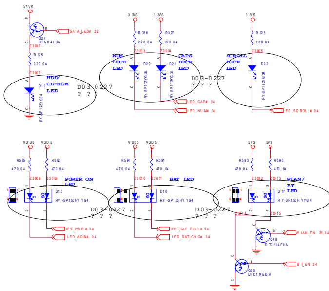
LED
