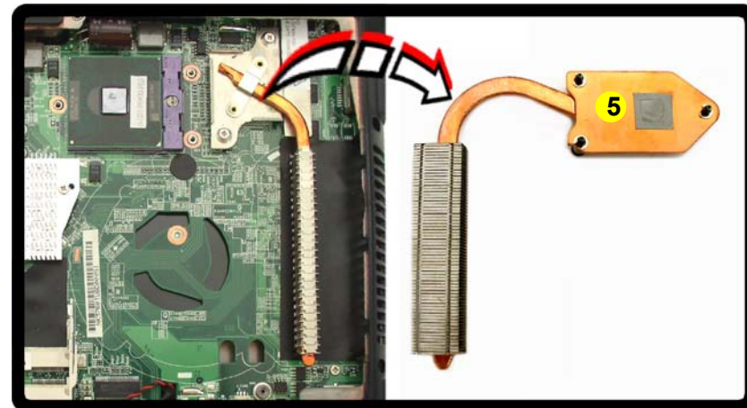
M760T/M760TU
