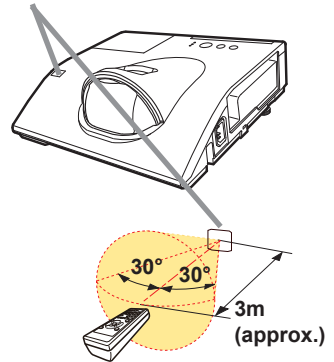
Remote sensor
