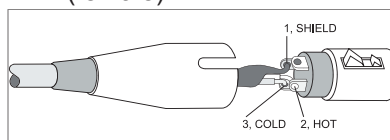
XLR (female)
