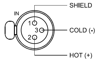
Illustration 4.4: Pin-assignment of AES/EBU-IN
