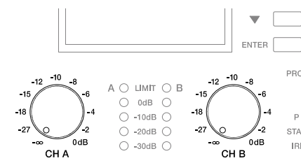
Illustration 3.1: Level controls CH A and CH B
