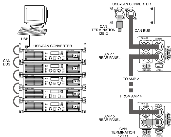
Illustration 4.10: System with 5 power amps (with RCM-26) and 1 USB-CAN-Converter. Termination plugs at the USB-CAN-Converter and the RCM-26 of amp 5
