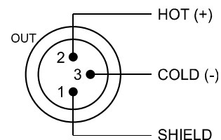
Illustration 4.5: Pin assignment of AES/EBU-OUT
