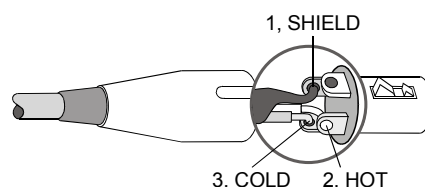
Illustration 2.12: Balanced connection of output (Daisy-Chain)
