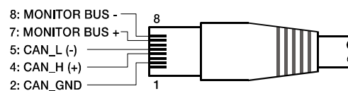
Illustration 4.7: Pin-assignment of CAN plug
