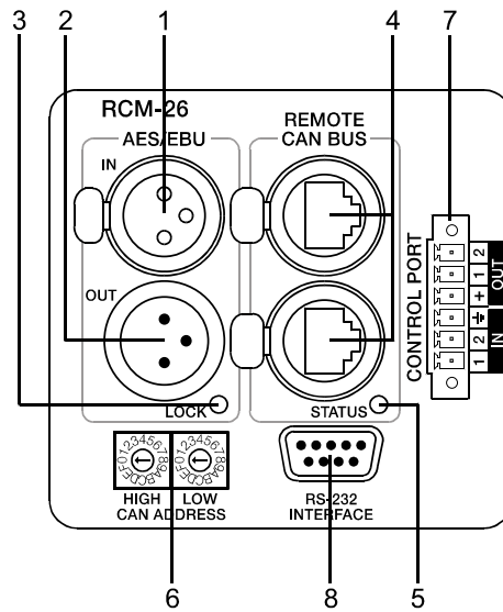
Illustration 4.3: Controls and Connections of the RCM-26
