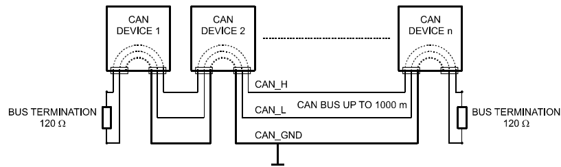
Illustration 4.9: Bus Topology of the CAN bus
