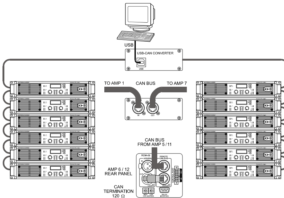
Illustration 4.11: System with 2 amp-racks and 1 USB-CAN-Converter. Termination plugs at amp 6 (first unit on the bus) and amp 12 (last unit on the bus)
