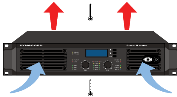
Illustration 2.6: H2500/H5000 Ventilation
