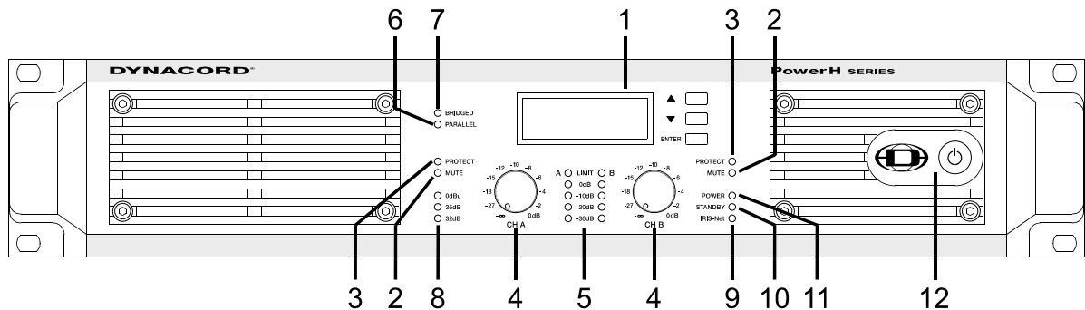
Illustration 2.1: H2500/H5000 front view
