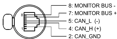
Illustration 4.6: Pin-assignment of CAN jack
