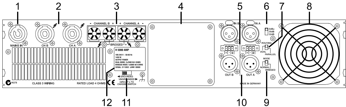
Illustration 2.2: H2500/H5000 rear view
