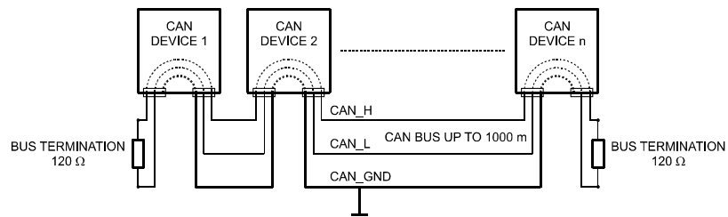
Illustration 4.9: Topologie du bus CAN
