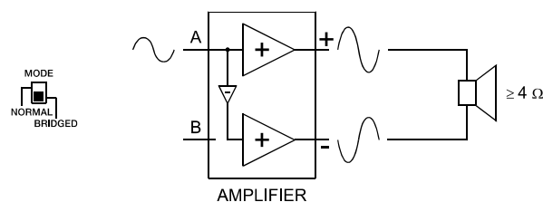
Illustration 2.9 : Mode BRIDGED
