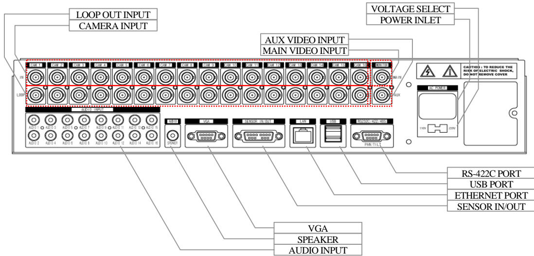
[Fig 5-2 Rear View]
