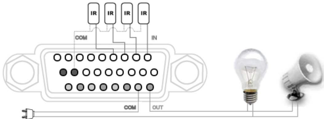
[Fig 5-6 RELAY OUT Connection]
