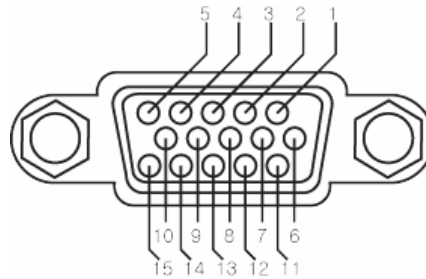
[Fig 5-4 VGA Connector PIN]
