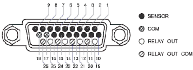
[Fig 5-5 SENSOR IN/OUT PIN]
