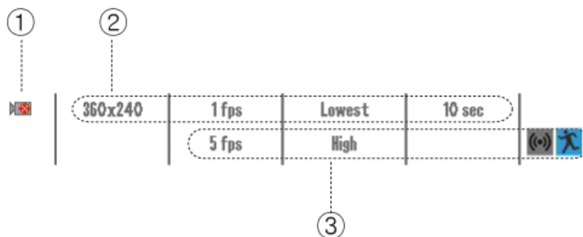
Figure 80 Recording Configuration
