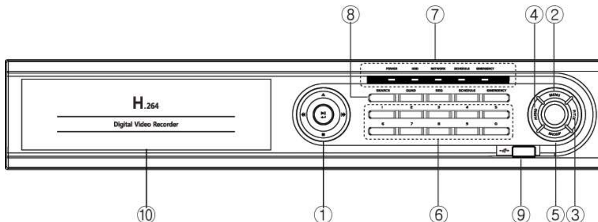
Figure 26 Front Panel
