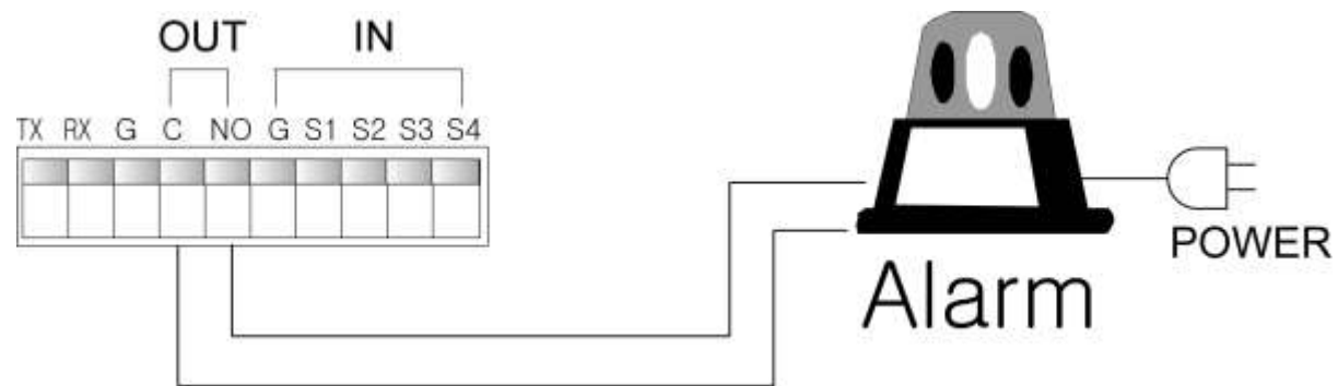
Figure 16 Alarm Out
