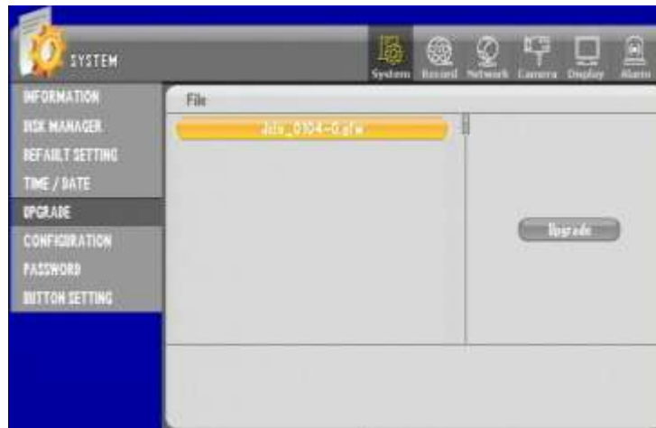
Figure 69 UPGRAD GUI
