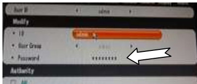
Figure 41 Password Field
