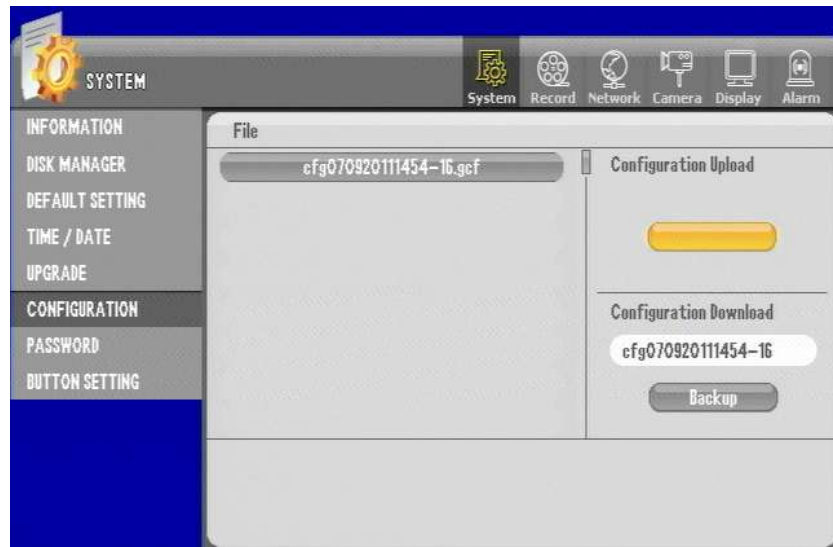
Figure 71 Configuration GUI
