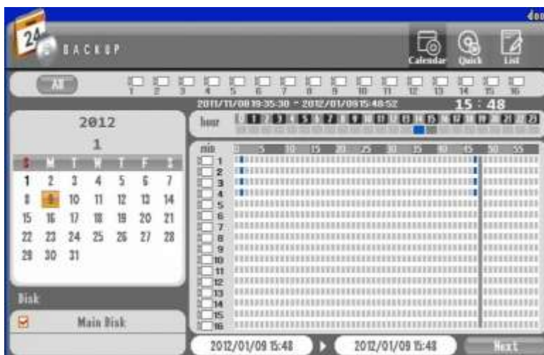
Figure 158 Calendar Backup
