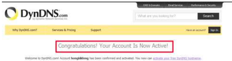
Figure 92 Active Notification
