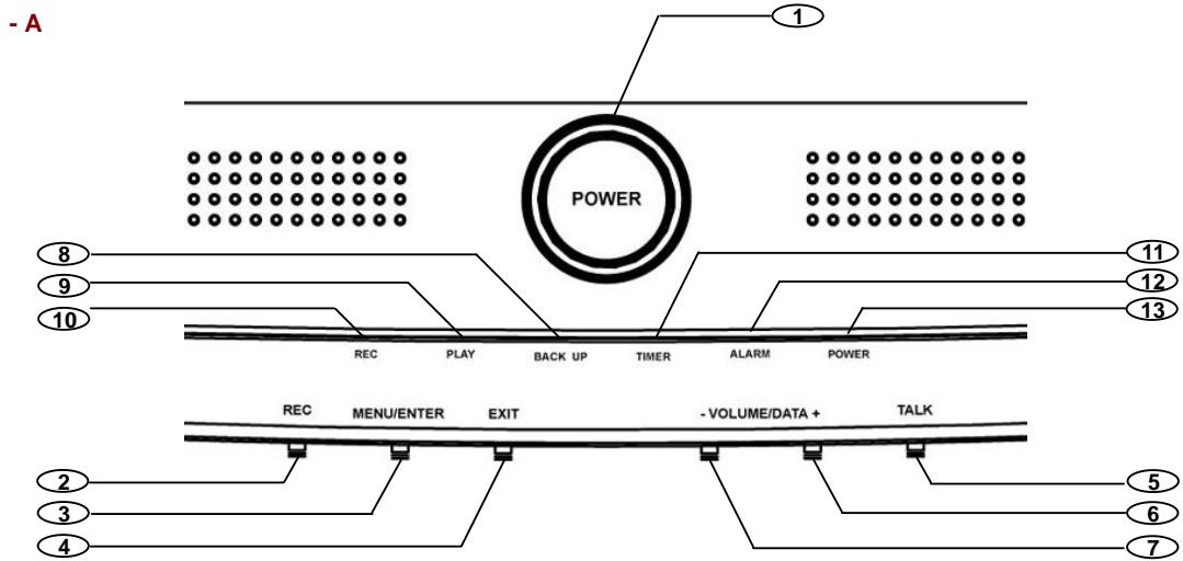
[Fig. 5-1 Front View]
