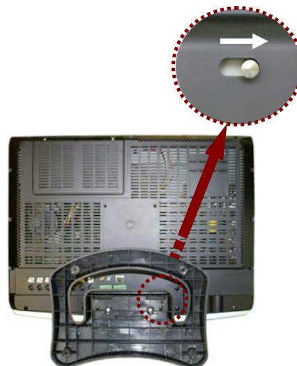
[Fig. 5-3-2 Locking the Lever]
