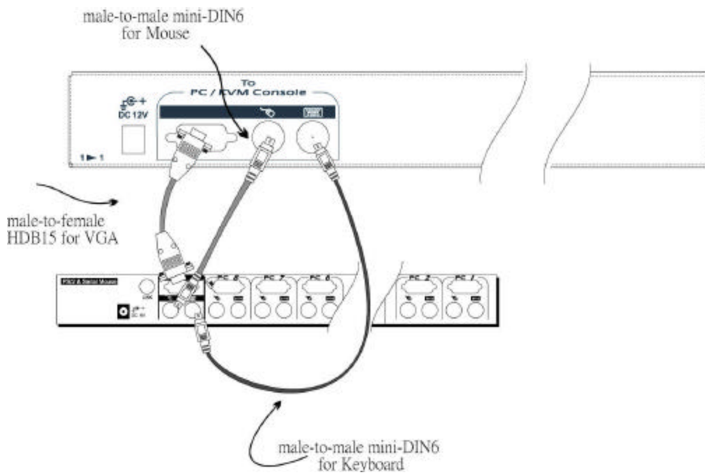
StreamLine Console connects to a Master-IT PRO KVM switch
