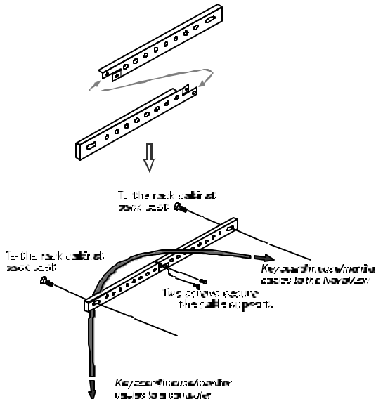
Figure 4. Rear Cable Support Bar.
