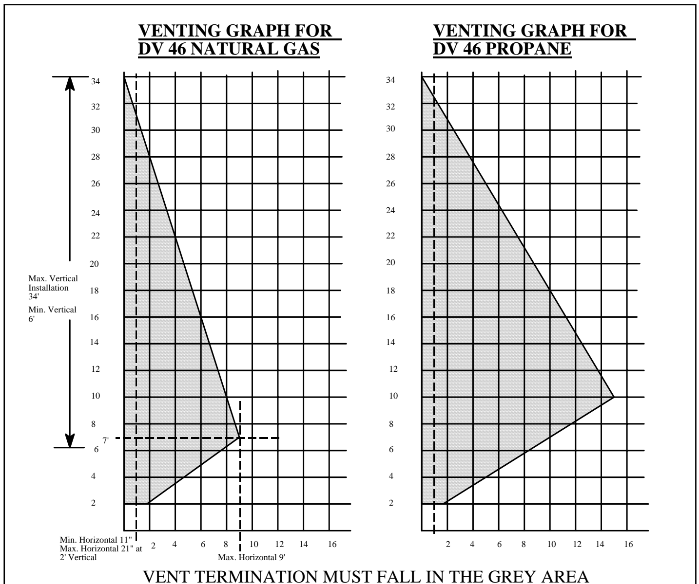
FIGURE 18: BAYVUE DV VENT GRAPHS, MODEL DV 46
