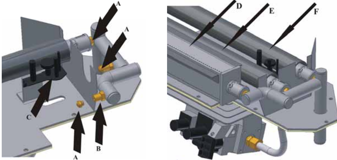
FIGURE 25: BURNER ASSEMBLY
