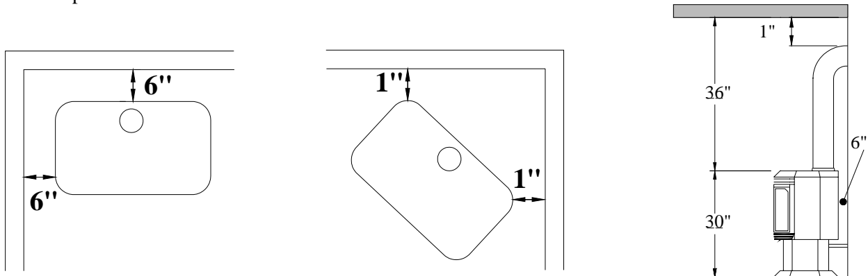
FIGURE 2: BAYVUE DV MINIMUM CLEARANCES
