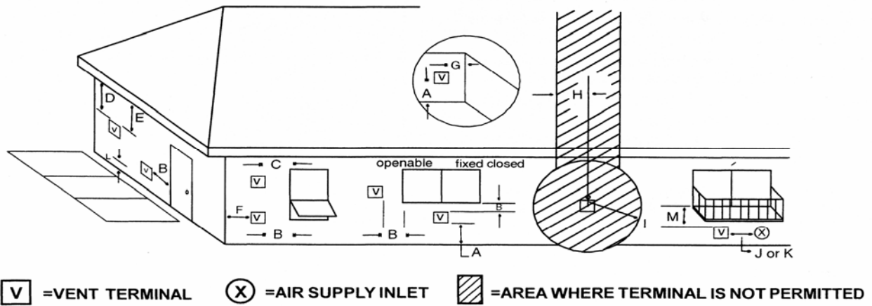
FIGURE 3: CLEARANCE REQUIREMENTS
