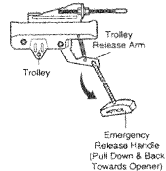
Lockout position
