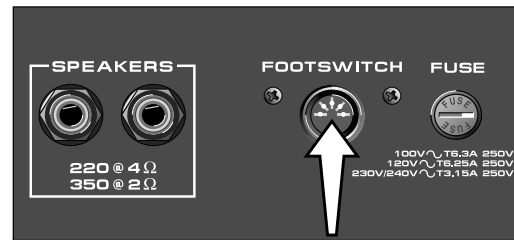
VTX350H REAR PANEL
