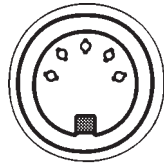
AT style 5 PIN DIN Connector
