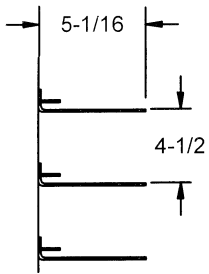
DETAIL OF PAN SLIDE
