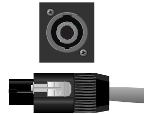
Figure 2.5 Top: Speakon Connector on Amplifier. Bottom: Speakon Cable Connector.
