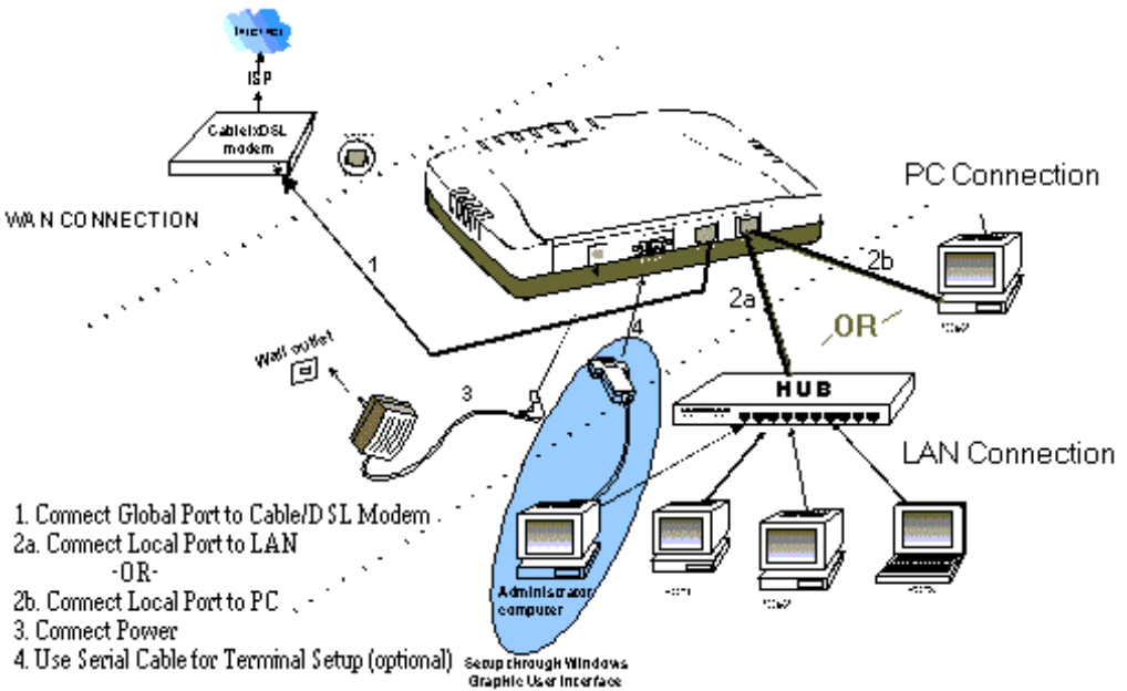
Figure 2: Hardware Connections
