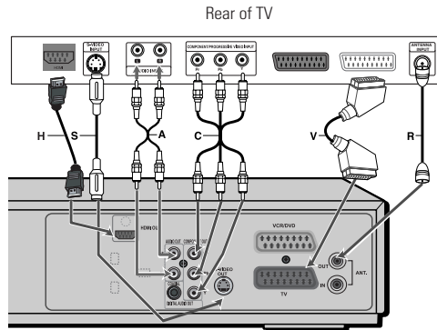
Rear of DVB-T VCR/DVD Recorder
