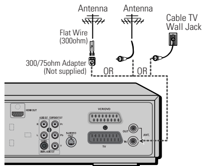
Rear of DVB-T VCR/DVD Recorder
