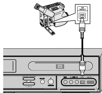
Front of DVB-T VCR/DVD Recorder
