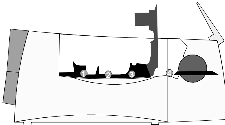
Figure 4-8: Clean rollers in the card track
