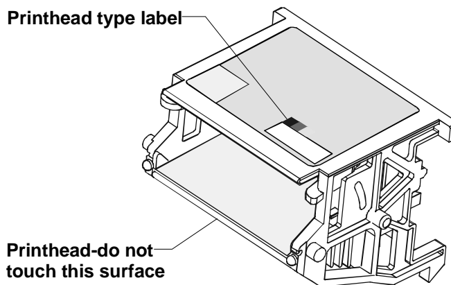
Figure B-6: Select replaceable printhead cartridge
