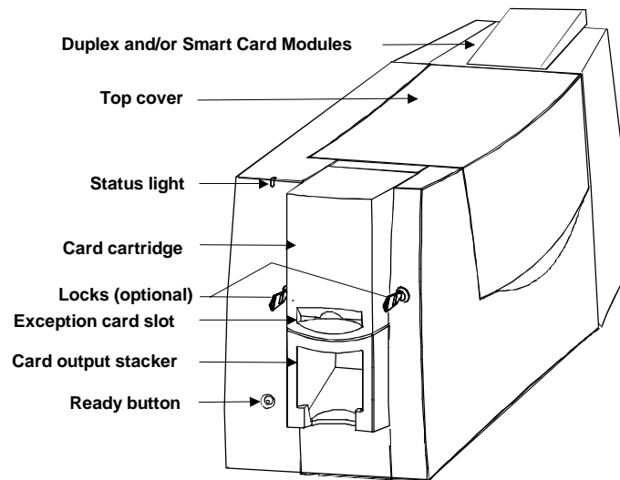
Figure 1-3: Front of the Select printer
