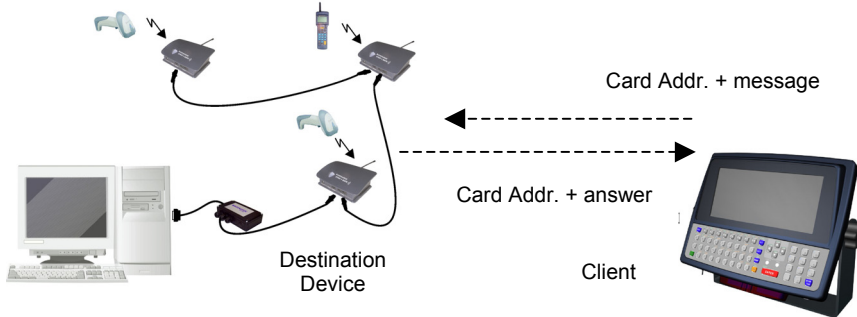
Figure 10 - Transmitting a Message in 2 Way Mode
