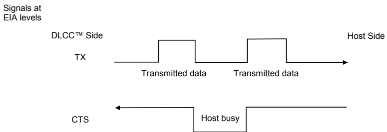
Modem RTS/CTS Handshaking
