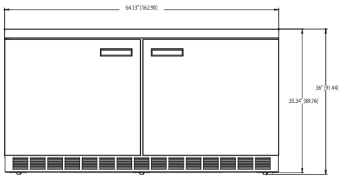
4464N ELEVATION VIEW
