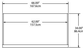
PLAN VIEW SSHRI2-S, SAHRI2-S, SMHRI2-S
