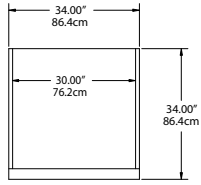
PLAN VIEW SSHRI1-S, SAHRI1-S, SMHRI1-S
