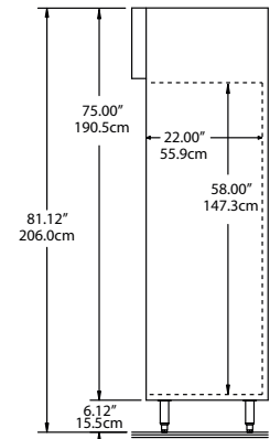
END VIEW ALL MODELS
