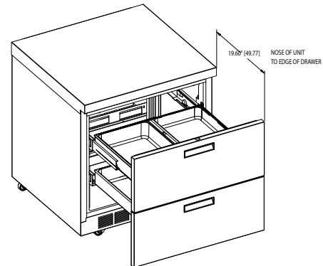
UCD4432N ISO View
