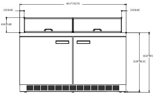
UC4460N-24M ELEVATION VIEW
