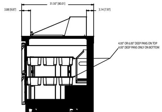
UCD4460N-18M RIGHT SIDE VIEW
