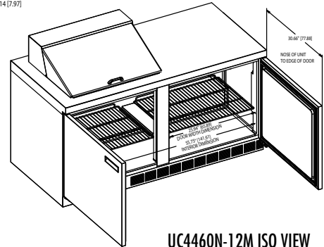
UC4460N-12M ISO VIEW
