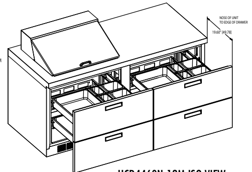
UCD4460N-12M ISO VIEW
