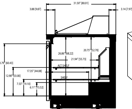
UC4460N-12M RIGHT SIDE VIEW
