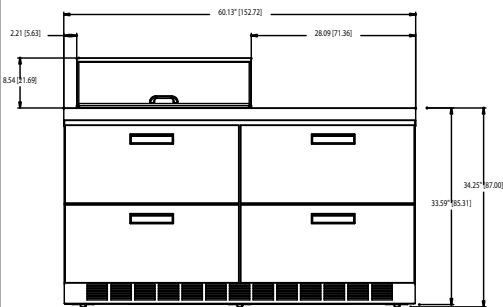
UCD4460N-12M ELEVATION VIEW
