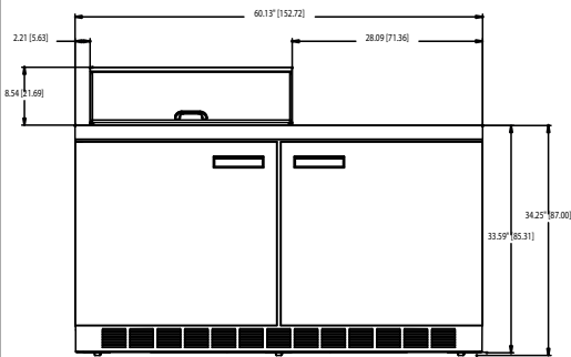
UC4460N-12M ELEVATION VIEW
