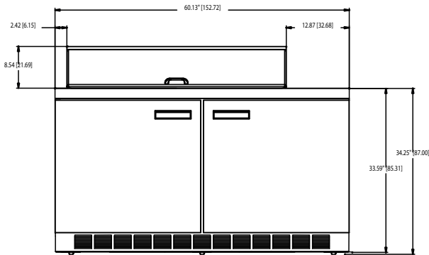
UC4460N-18M ELEVATION VIEW
