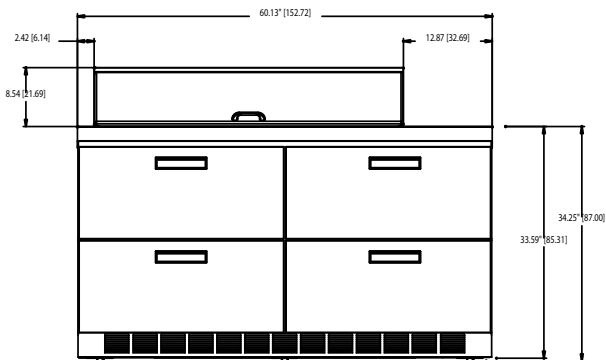
UCD4460N-18M ELEVATION VIEW
