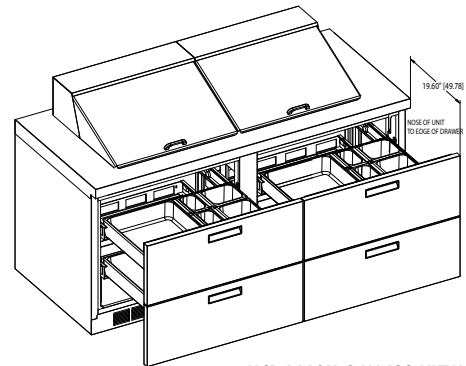
UCD4460N-24M ISO VIEW
