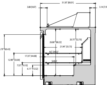
UC4460N-24M RIGHT SIDE VIEW
