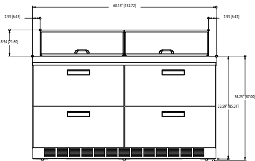
UCD4460N-24M ELEVATION VIEW
