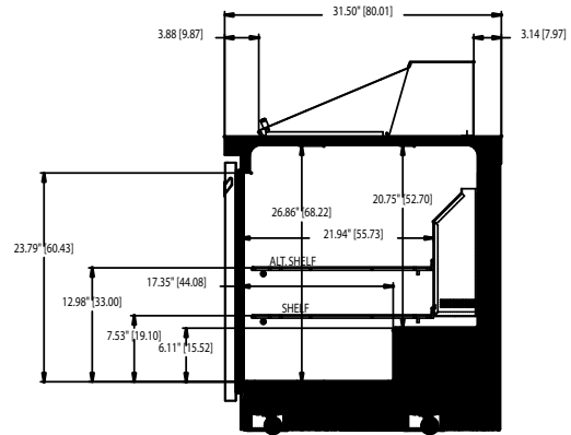
UC4460N-18M RIGHT SIDE VIEW
