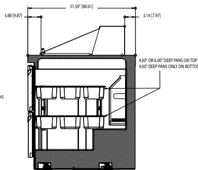
UCD4460N-24M RIGHT SIDE VIEW
