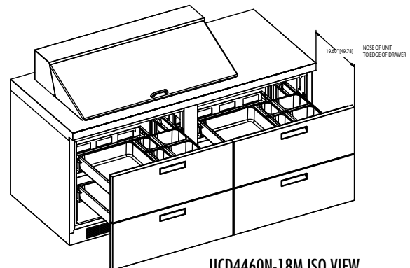
UCD4460N-18M ISO VIEW
