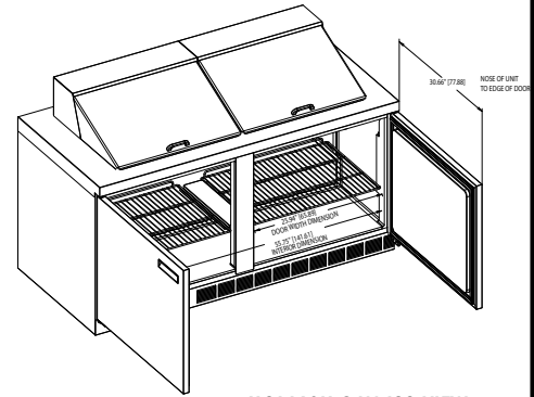
UC4460N-24M ISO VIEW
