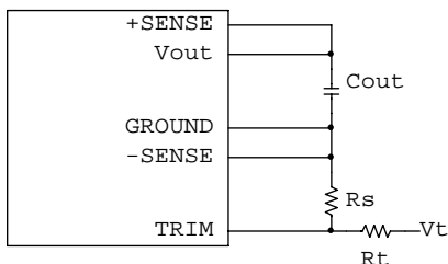
Figure 33: Output voltage trim with voltage source DS_NC12S30A_05222008
