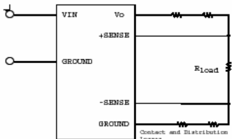
Figure 25: circuit configuration for remote sense
