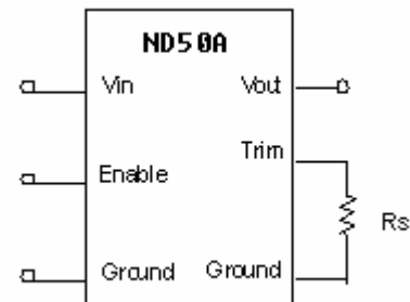
Figure 26: Trimming Output Voltage
