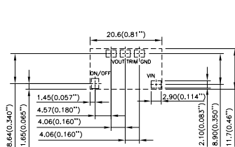
RECOMMEND PWB PAD LAYOUT
