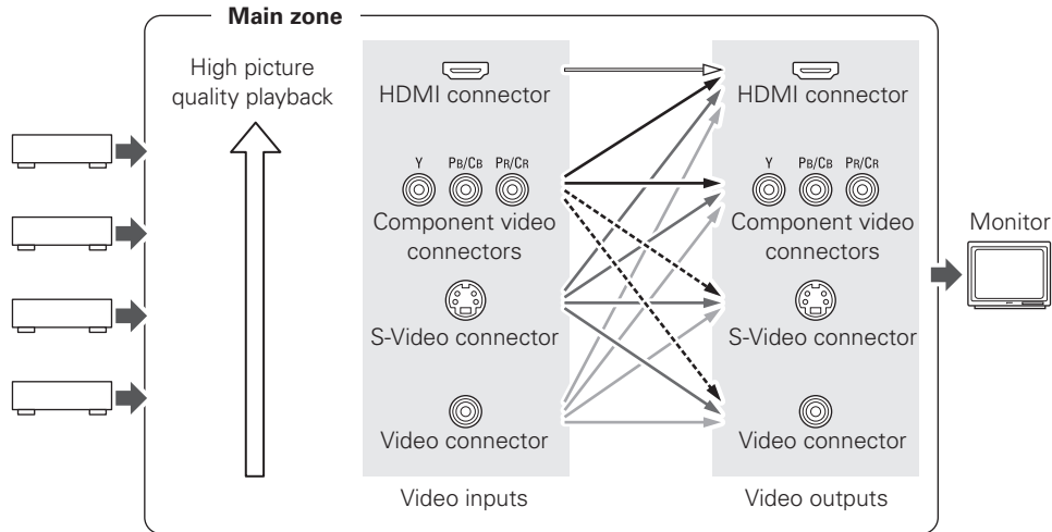
[Flow of video signals inside the AVR-2308CI]
