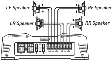
4 Channel Mode, 1 speaker per channel
