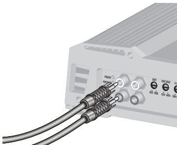
Source Unit Audio Cables Connected to the RCA Inputs
