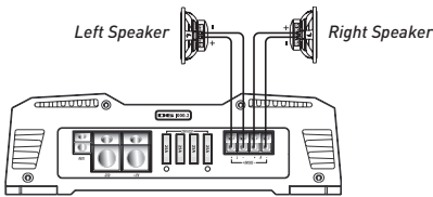
2 Channel Mode, 1 speaker per channel
