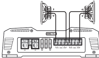
2 Channel Mode, both pairs of channels bridged
