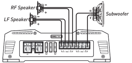
3 Channel Mode, 1 pair stereo plus one bridged channel
