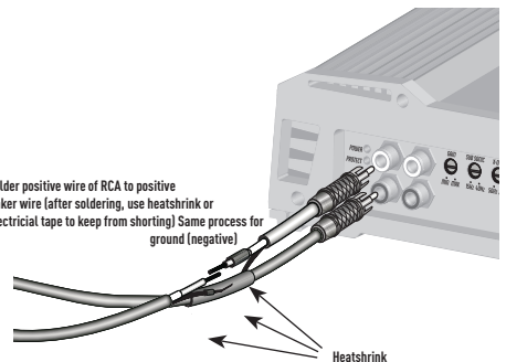
Speaker Wires from the Factory Audio System Connected to the High Level Inputs
