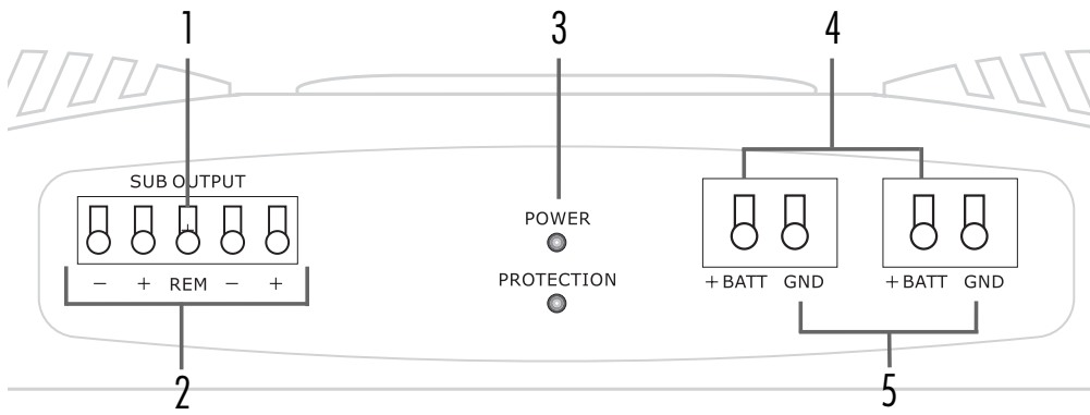
FIGURE 2—AMPLIFIER CONNECTIONS d2500.1 REAR
