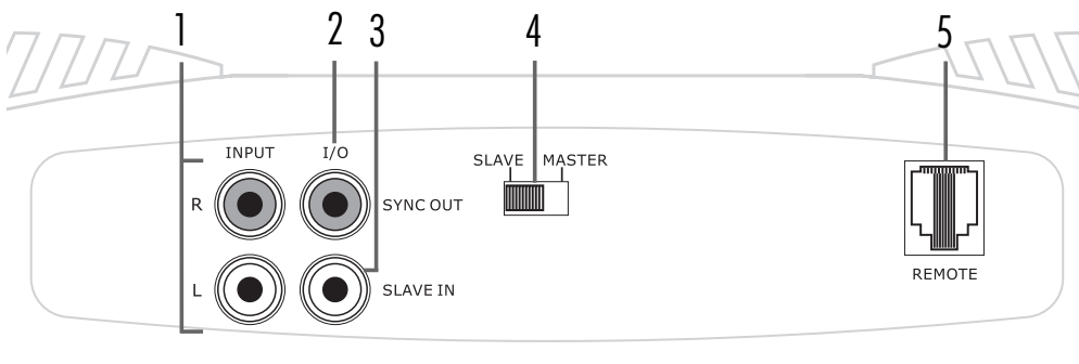
FIGURE 1—AMPLIFIER CONNECTIONS d2500.1 FRONT
