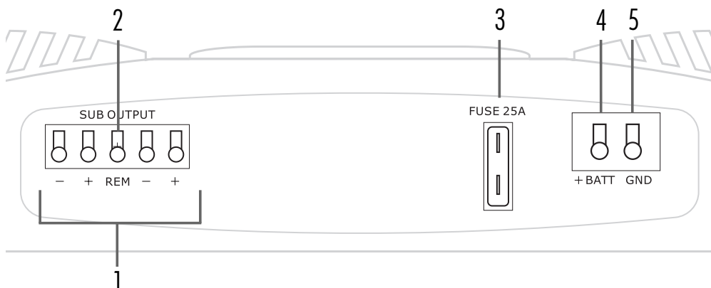
FIGURE 2—AMPLIFIER CONNECTIONS d300.1 REAR
