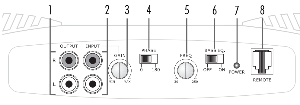
FIGURE 1—AMPLIFIER CONNECTIONS d300.1 FRONT
