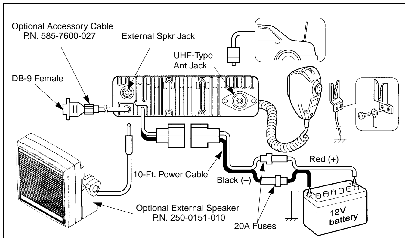
Figure 2-1 Installation Components
