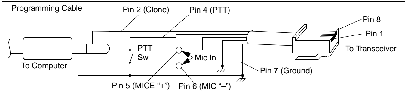
Figure 6-3 Test Cable Schematic
