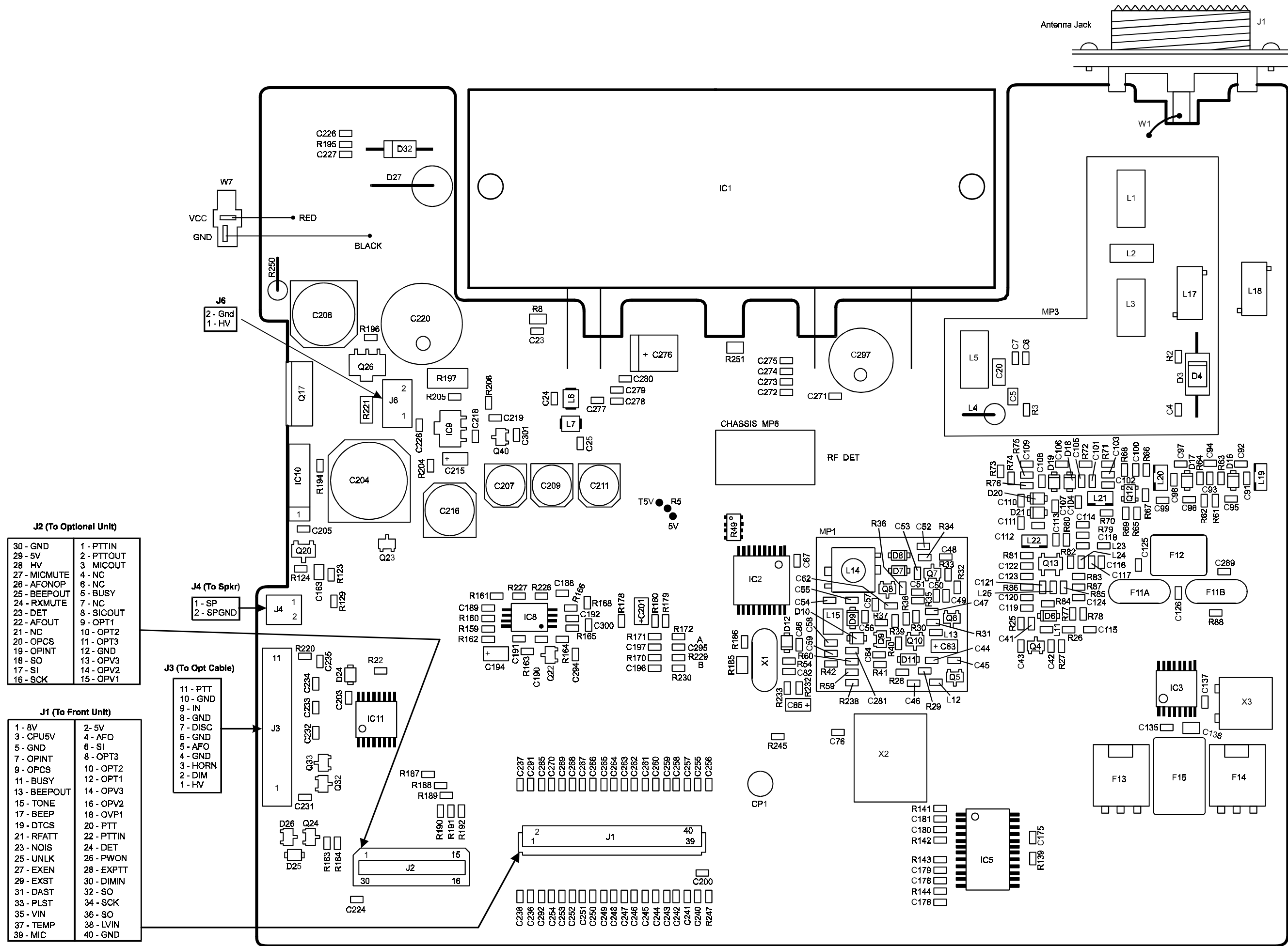
VHF (7610) MAIN BOARD TOP VIEW
