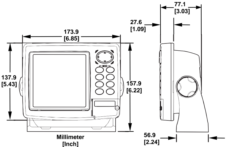
Front view (left) and side view (right) showing dimensions of the SeaCharter 640cDF unit when mounted on gimbal bracket.
