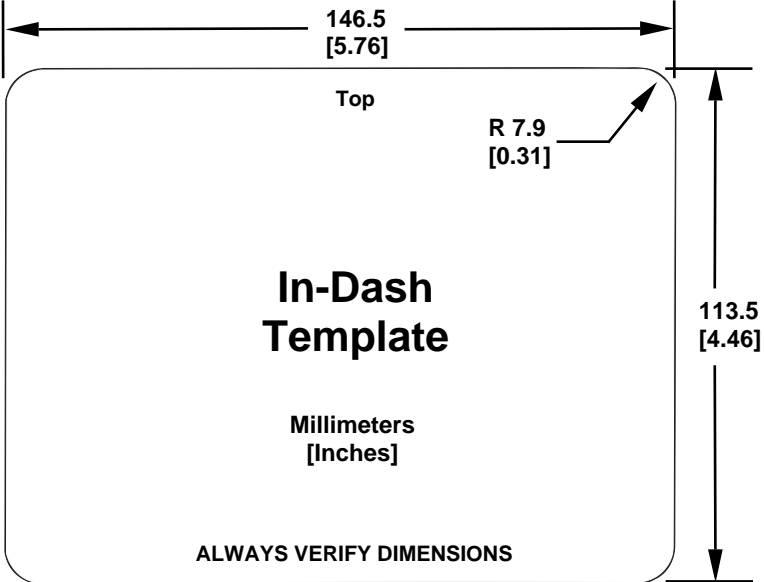
In-dash mounting template for SeaCharger 640cDF sonar/GPS unit, showing dimensions. NOTE: The figure above is not printed to scale. A scaled template (FM-5 In-Dash Adapter Kit instructions) is available for free download from our web site, www.eaglesonar.com .
