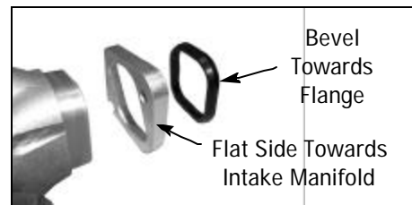
Manifold Flange Assembly Order (Apply Light Coat of Lube to Grommet)
