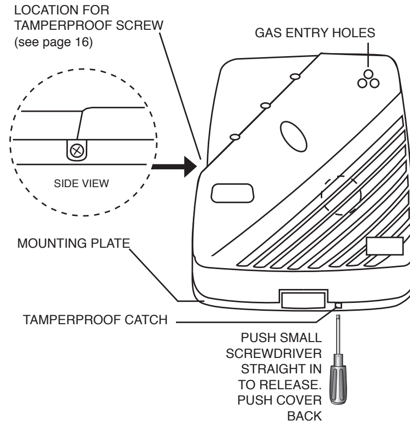
Figure 1 - Alarm Installation
