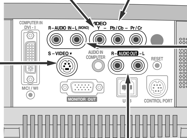
Terminals of the Projector
