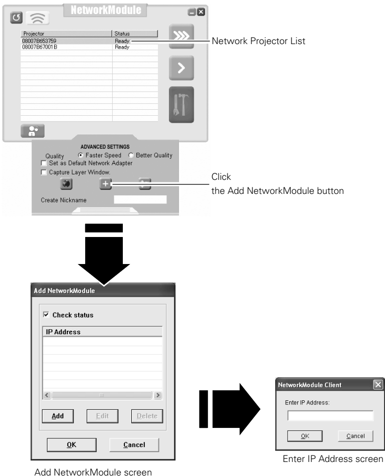
Add NetworkModule screen
