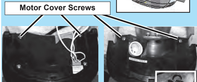
FIG. 5-2 Remove motor cover.
