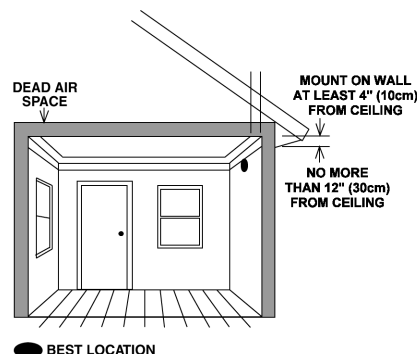
Figure 4: RECOMMENDED SMOKE ALARM MOUNTING LOCATIONS
